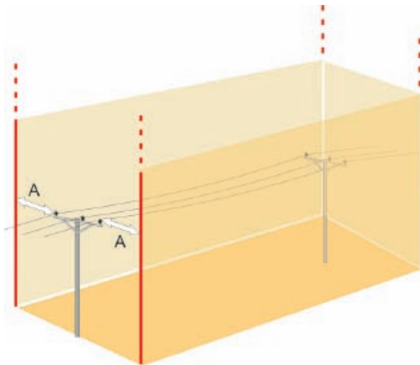
Fig 2. Hazard Zone
